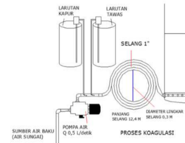
Gambar 1. Sketsa Proses Koagulasi Model Pipa Melingkar (Hamzani, 2013)
